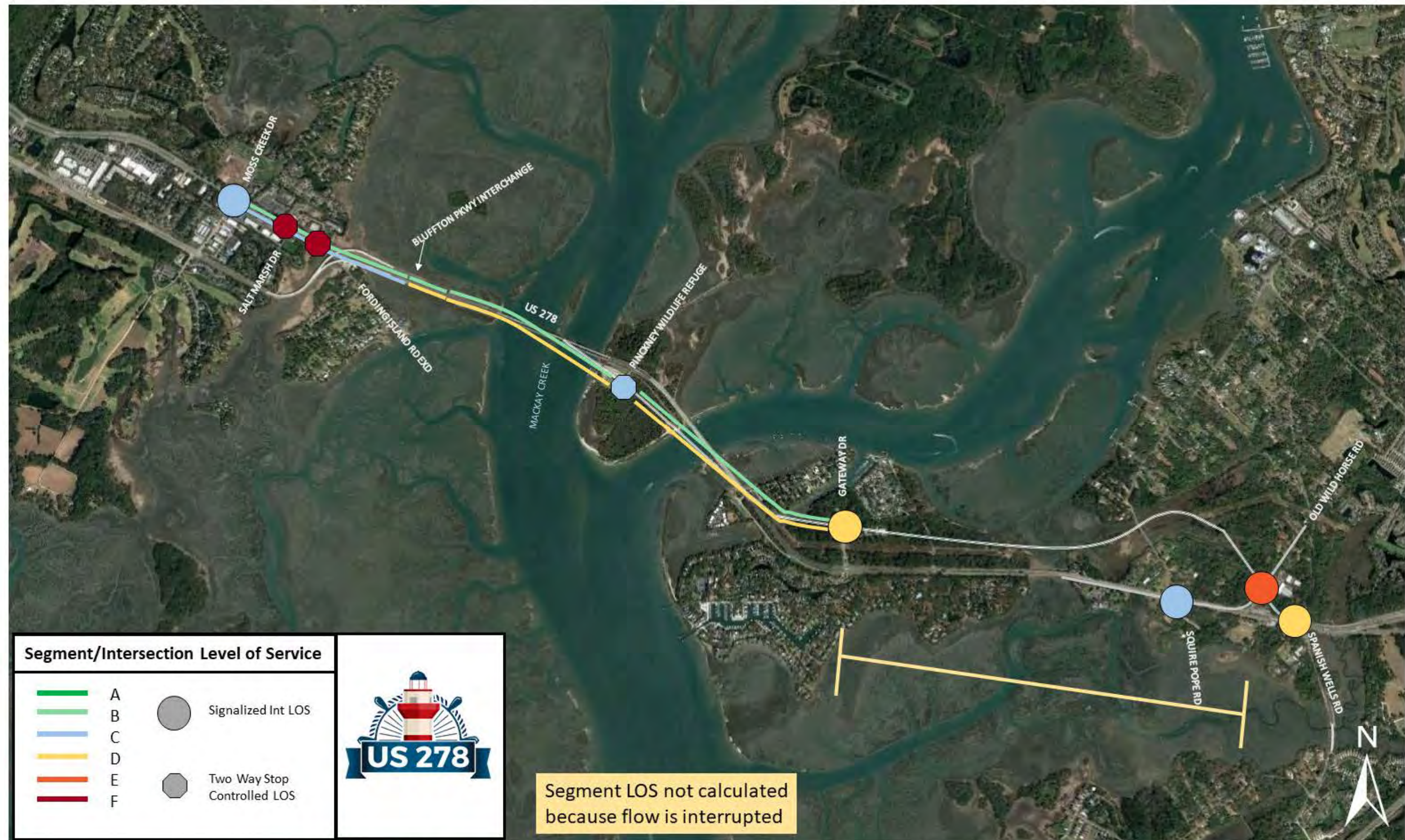
Figure 98: US 278 2045 Reasonable Alternative 6 AM Levels of Service Summary
