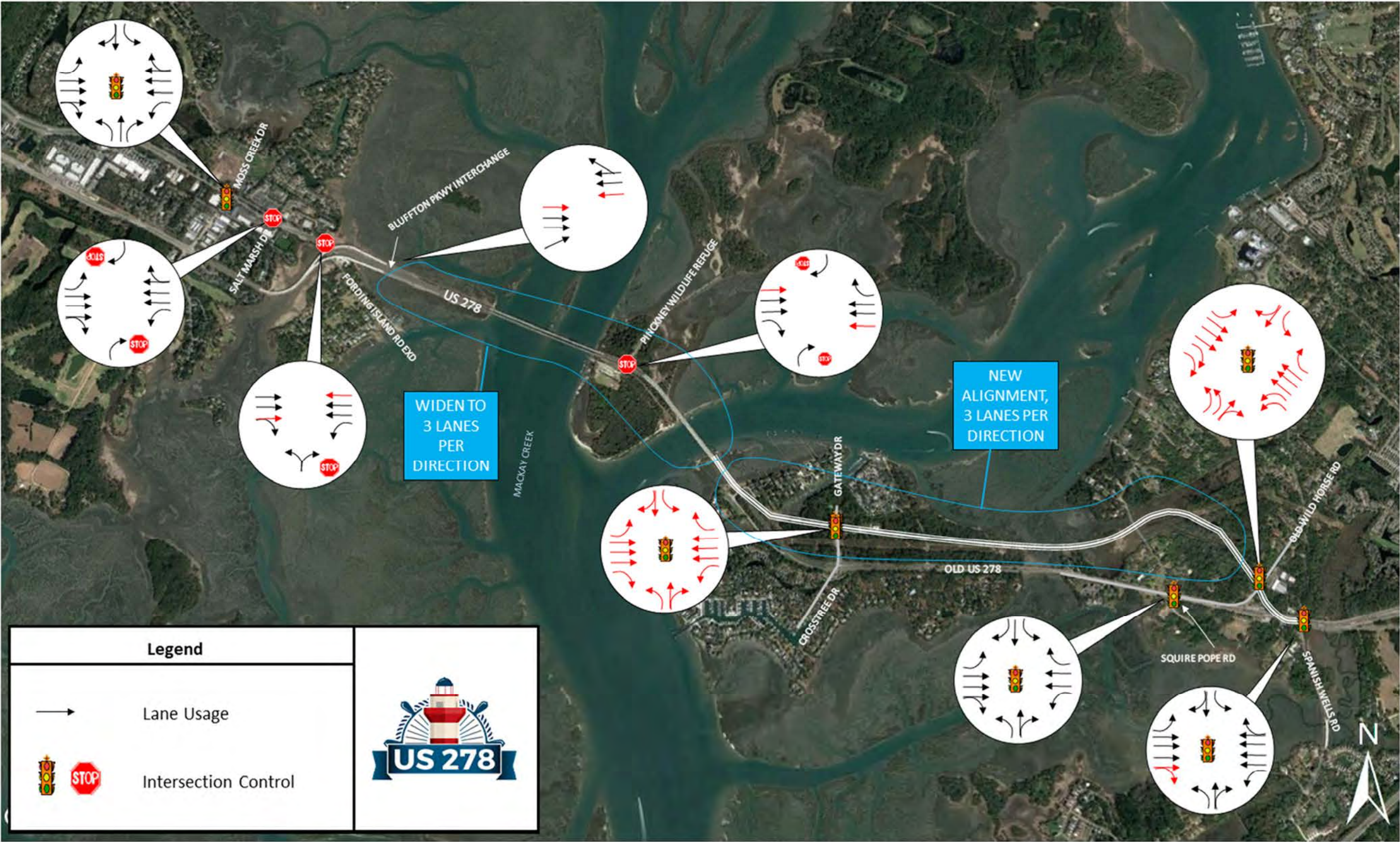
Figure 71: 2045 Reasonable Alternative 5 Geometric Layout
