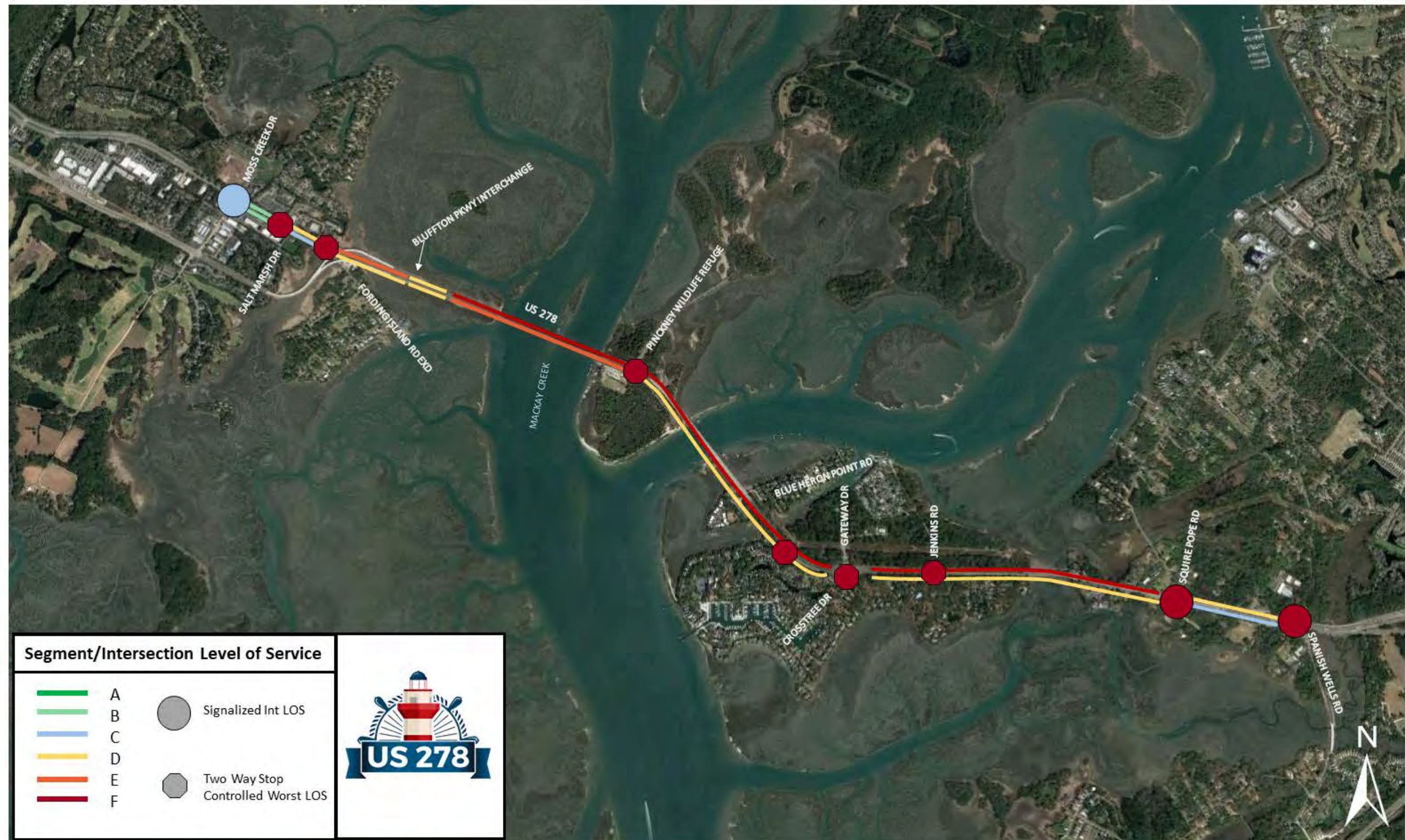
Figure 85: US 278 2045 No Build PM Levels of Service Summary (Excludes Jenkins Island Superstreet)
