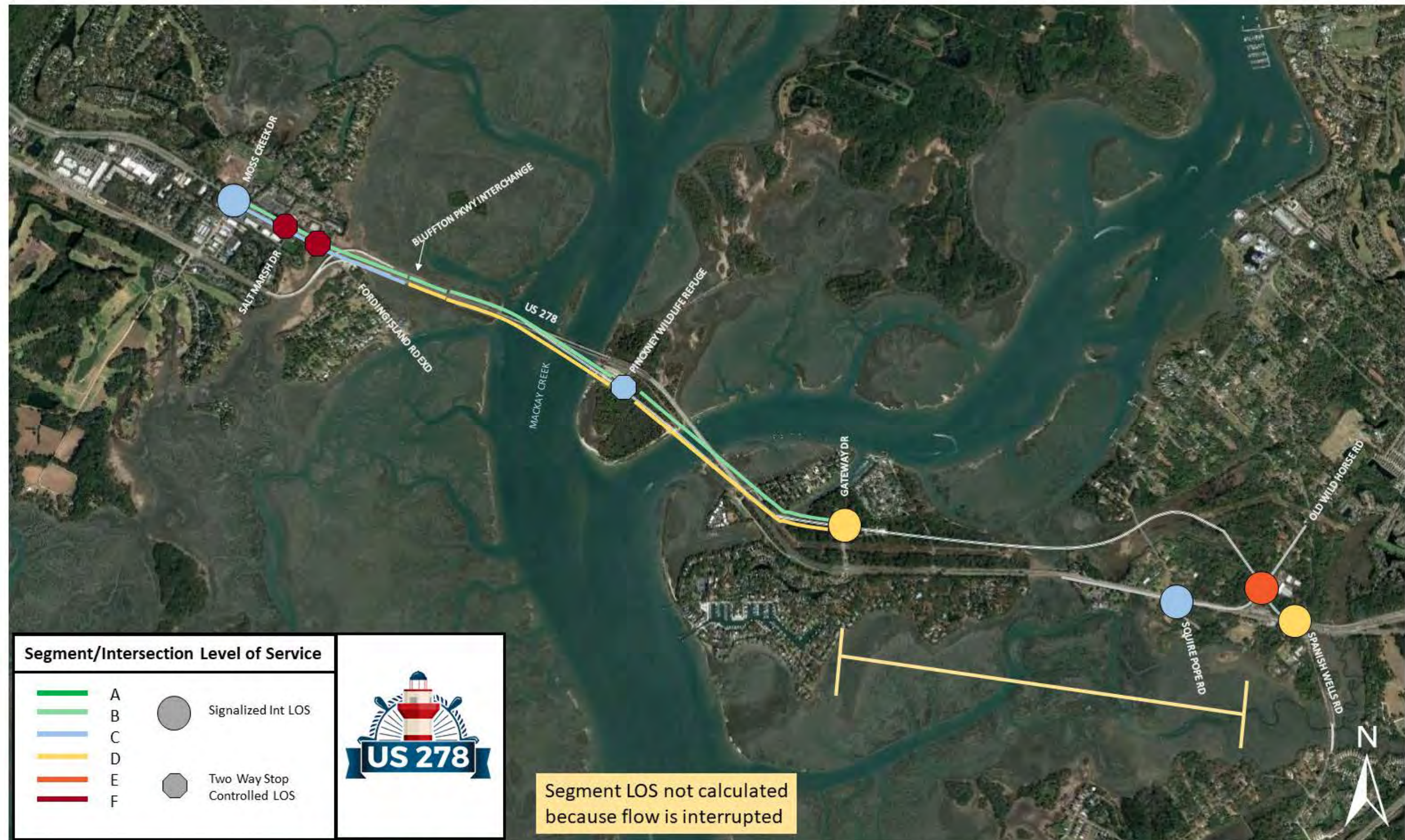
Figure 96: US 278 2045 Reasonable Alternative 5 AM Levels of Service Summary
