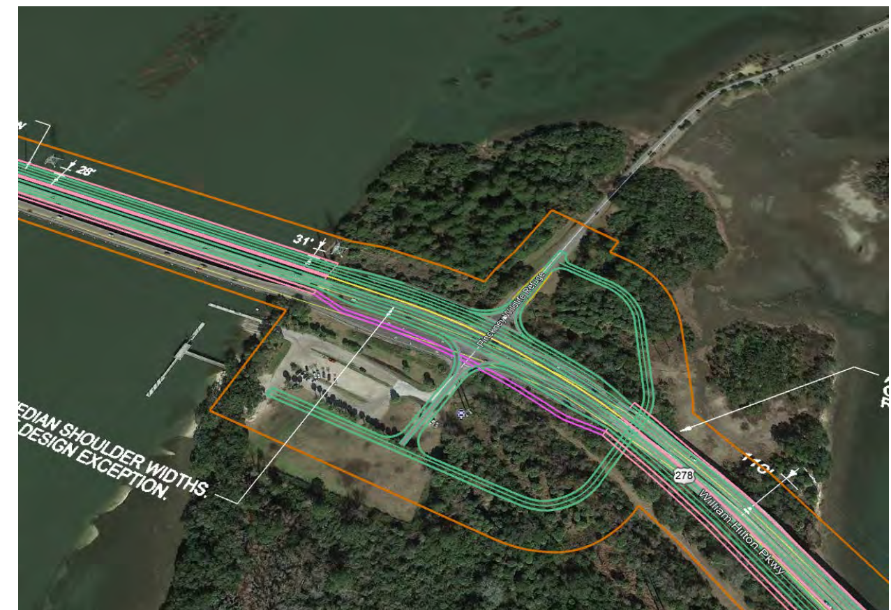
Figure 53: Pinckney Wildlife Refuge Interchange (included in all Reasonable Alternatives)
