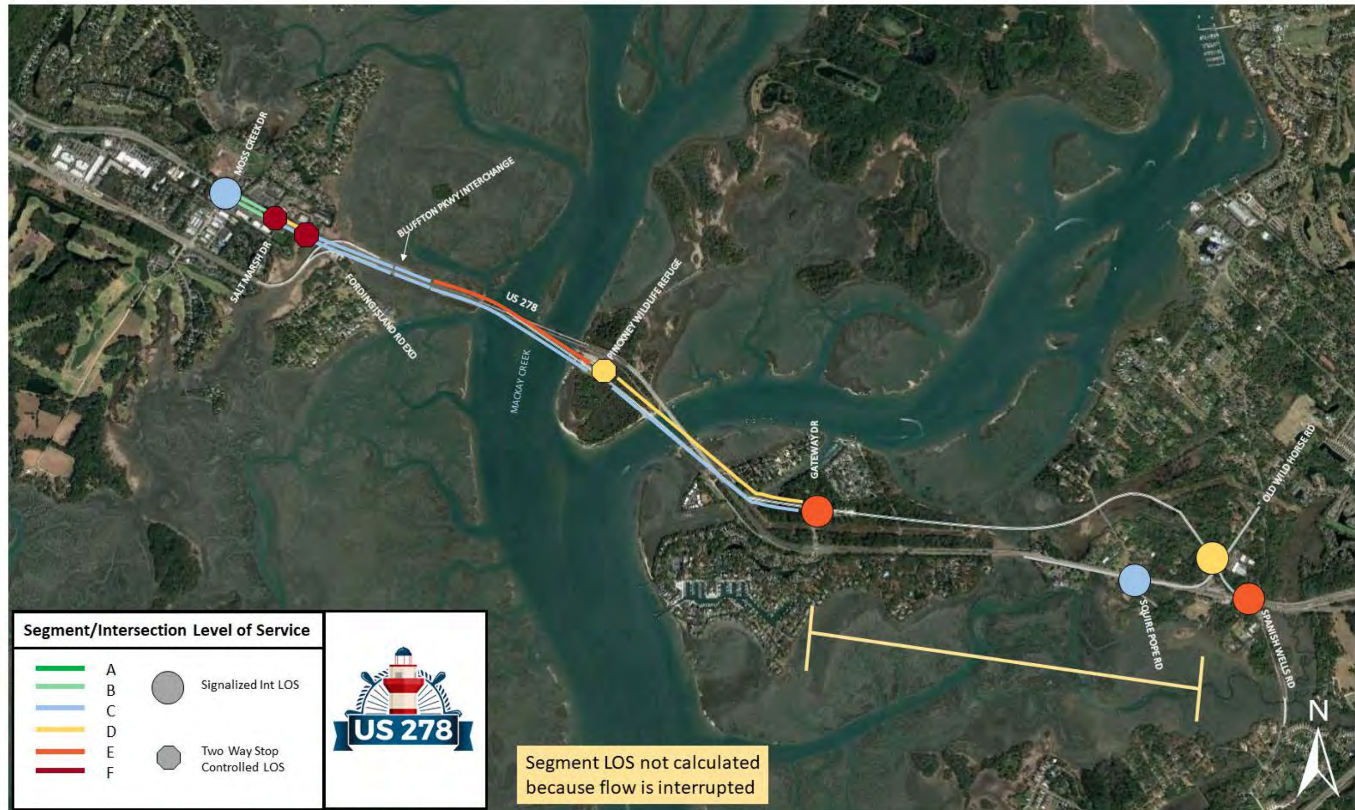
Figure 97: US 278 2045 Reasonable Alternative 5 PM Levels of Service Summary
